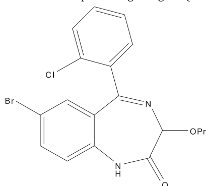
Scheme. Chemical structure of propoxazepam (I)
